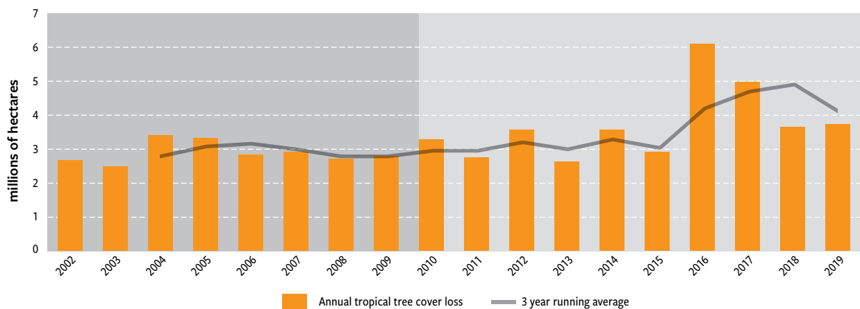
Figure 5.2. Loss of tree cover from tropical primary forests 3
