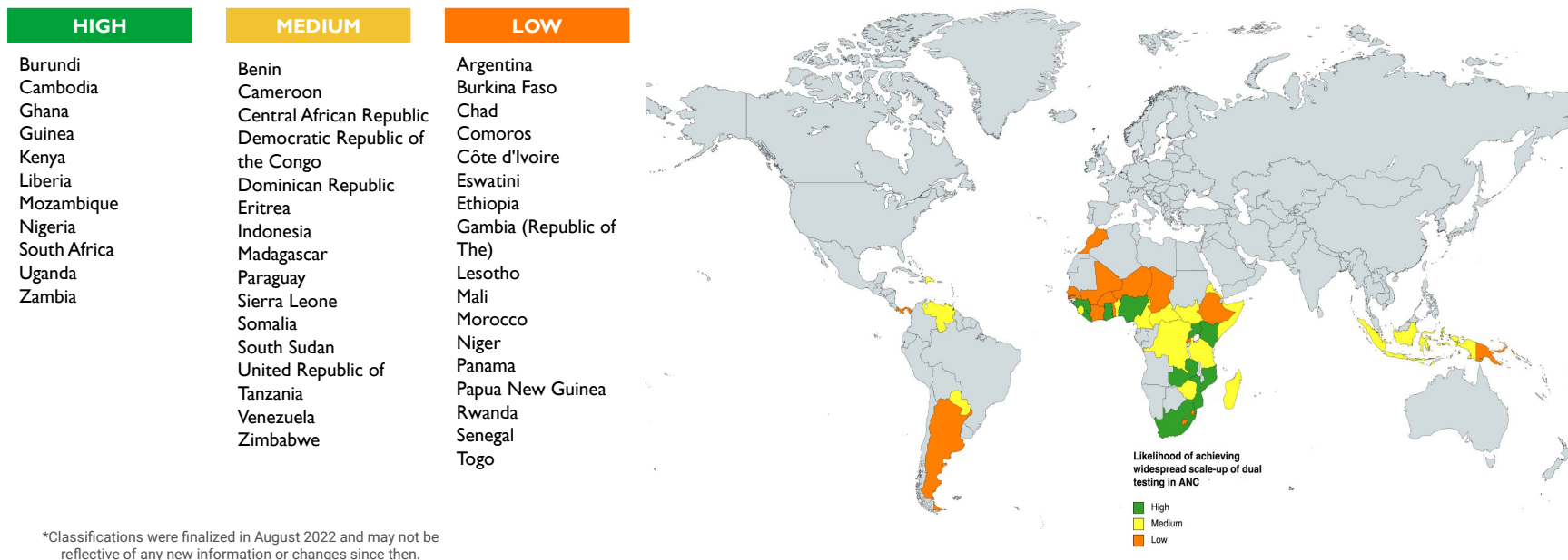
Figure 3.04: Global map of dual uptake classifications for LMICs
