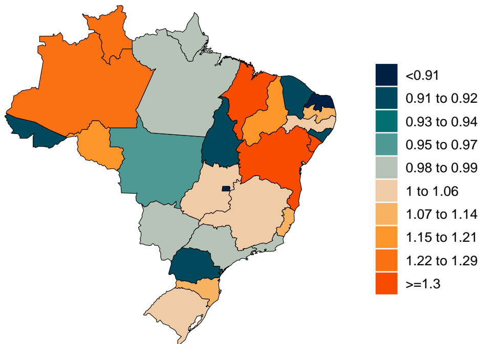
Figure 7.1: Mean effective R on June 30, 2022. Effective R less than 1 means that transmission should decline, all other things being held the same. The estimate of effective R is based on the combined analysis of deaths, case reporting, and hospitalizations where available. Current reported cases reflect infections 11-13 days prior, so estimates of effective R can only be made for the recent past.
