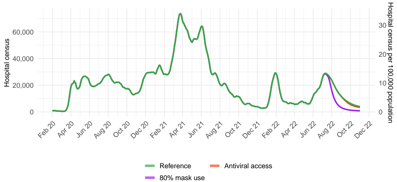
Figure 20.3: Daily COVID-19 hospital census until November 01, 2022 for three scenarios
