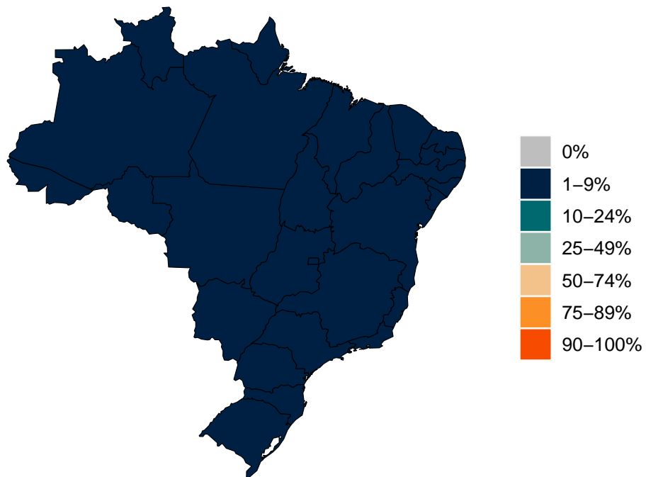
Figure 8.4: Estimated percent of new infections that are Gamma variant
