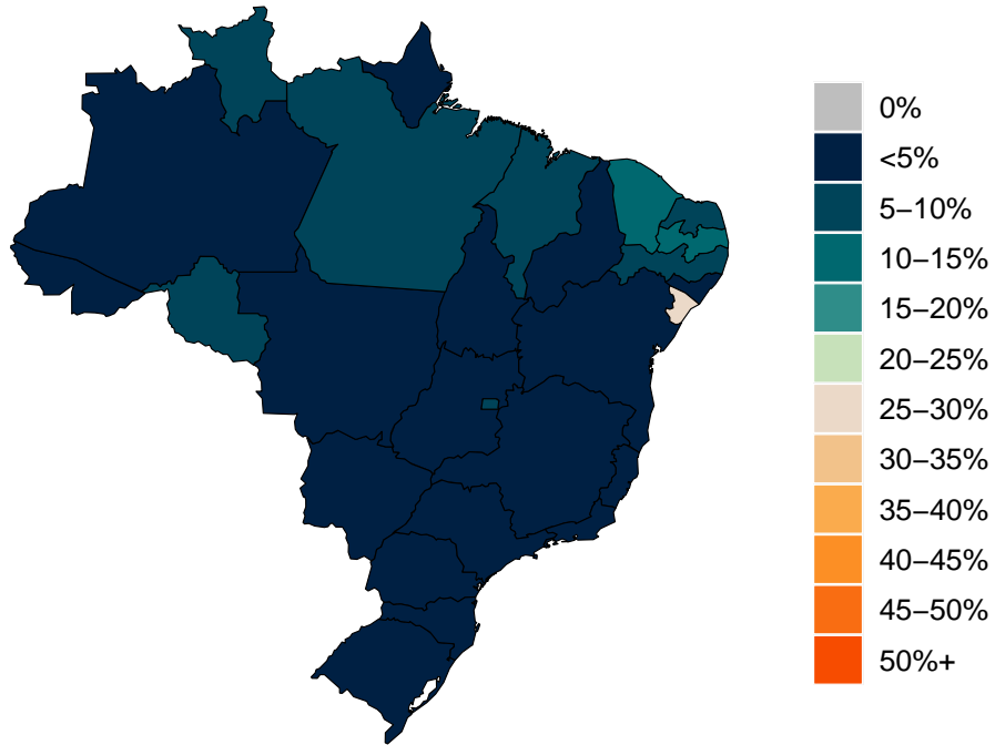
Figure 17.1: Estimated proportion of the total population that is not vaccinated but willing to be vaccinated as of June 24, 2022
