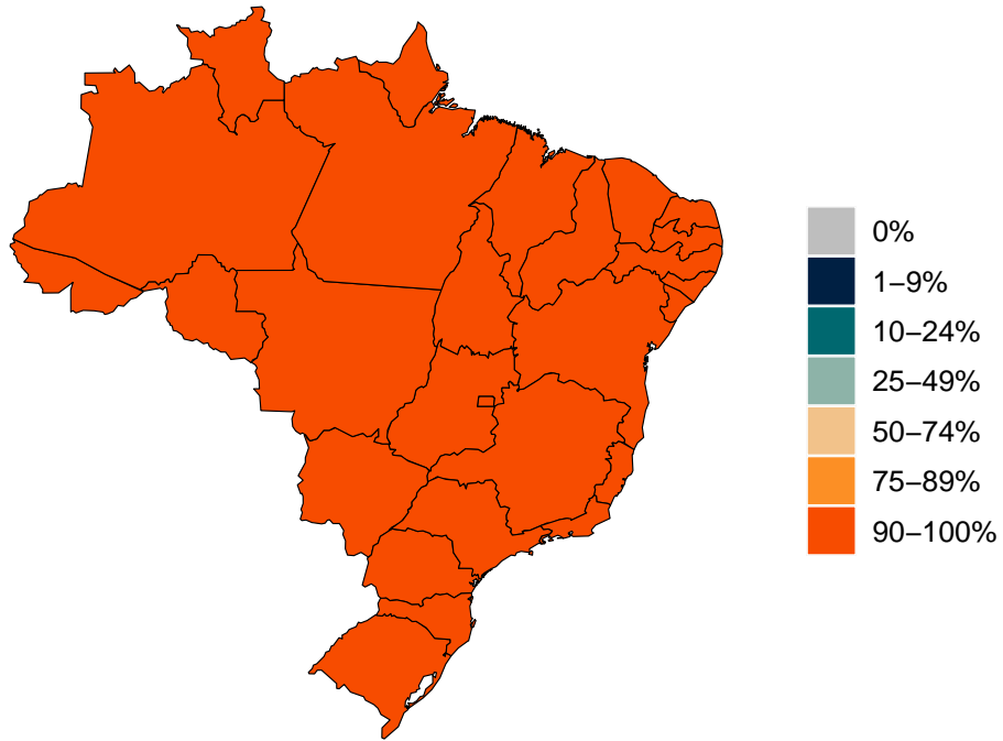
Figure 8.5: Estimated percent of new infections that are Omicron variant
