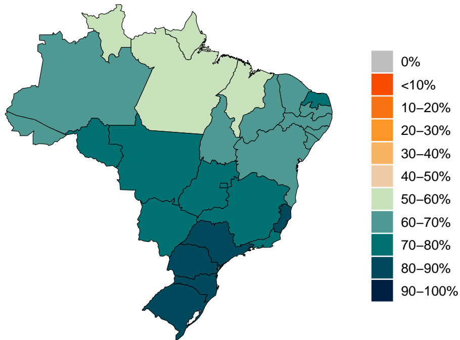
Figure 16.2: Percent of the population fully vaccinated against SARS-CoV-2
