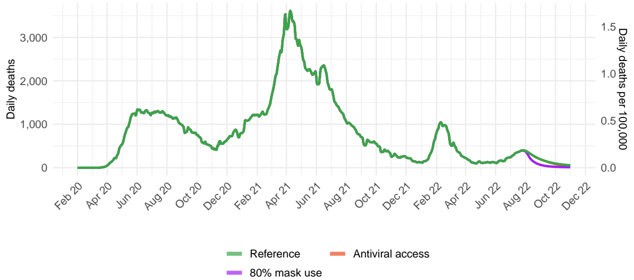
Figure 20.5: Total daily COVID-19 deaths per 100,000
