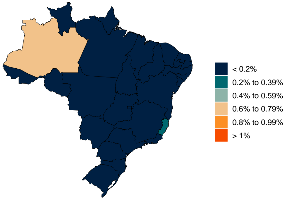
Figure 9.1: Infection-fatality rate on July 11, 2022. This is estimated as the ratio of COVID-19 deaths to estimated daily COVID-19 infections.
