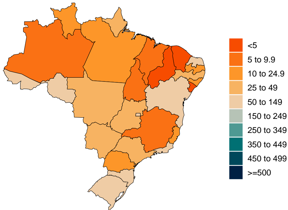
Figure 15.1: COVID-19 diagnostic tests per 100,000 people on July 11, 2022
