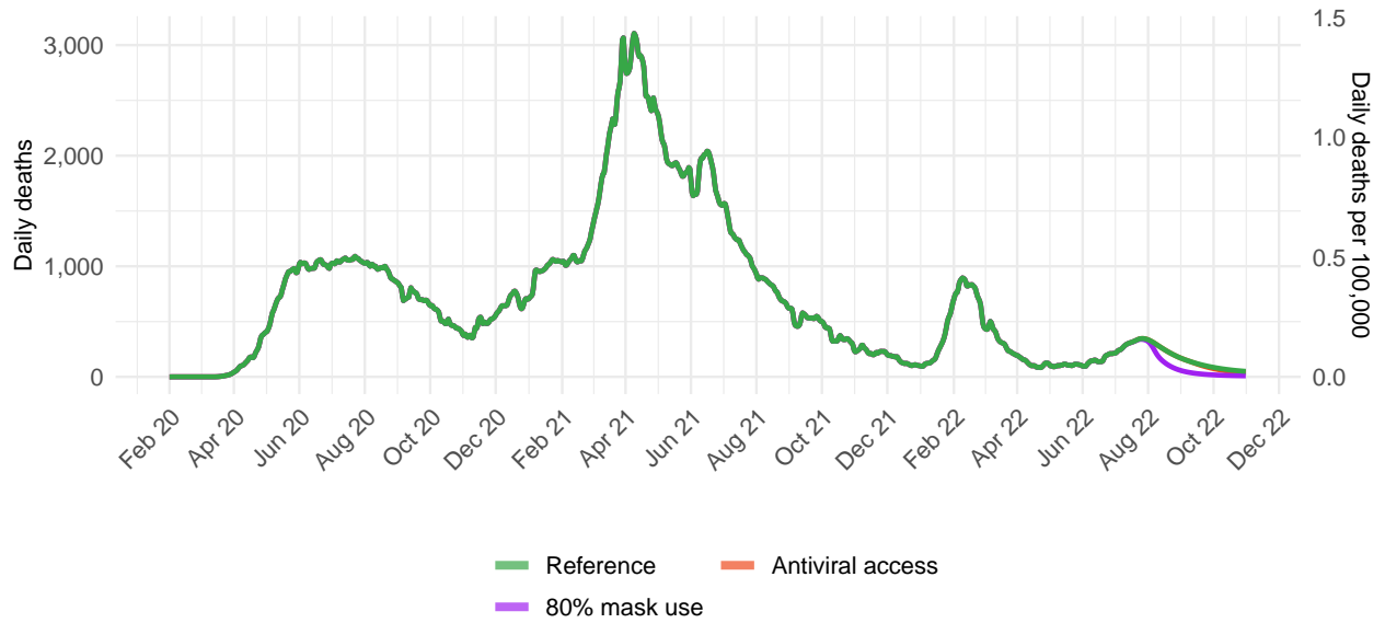
Figure 20.4: Reported daily COVID-19 deaths per 100,000
