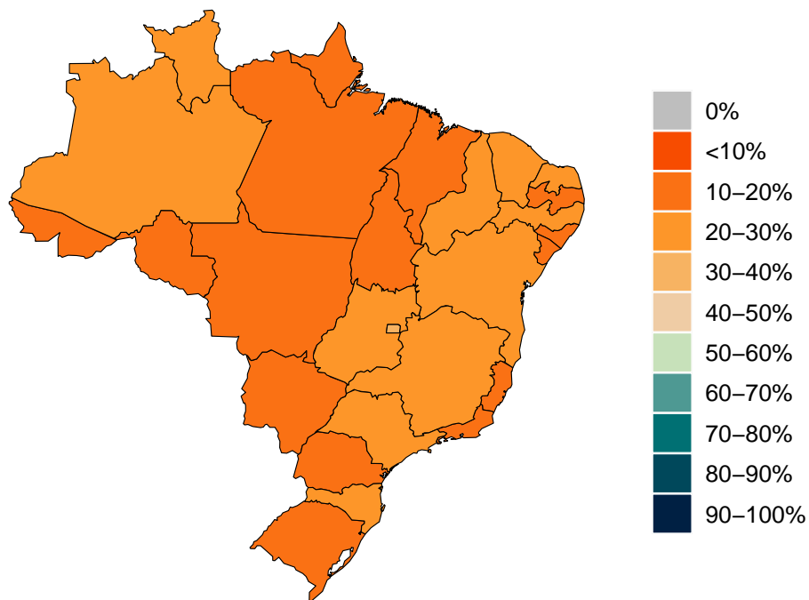
Figure 13.1: Proportion of the population reporting always wearing a mask when leaving home on July 11, 2022
