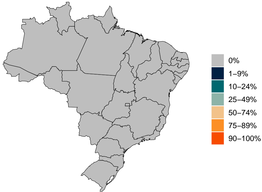
Figure 8.2: Estimated percent of new infections that are Beta variant
