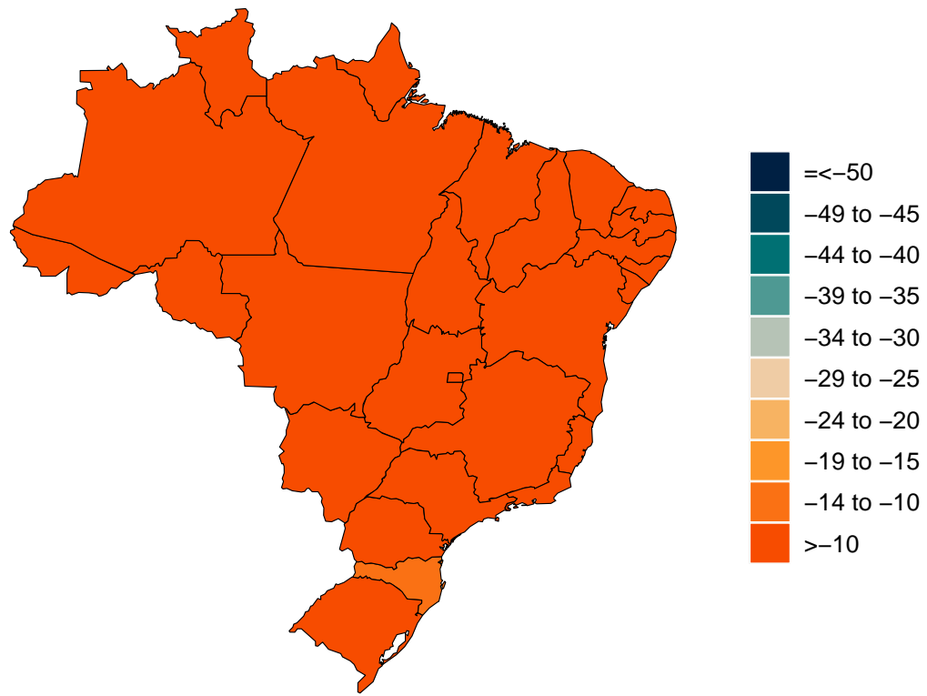
Figure 11.1: Mobility level as measured through smartphone app use, compared to January 2020 baseline (percent) on July 11, 2022
