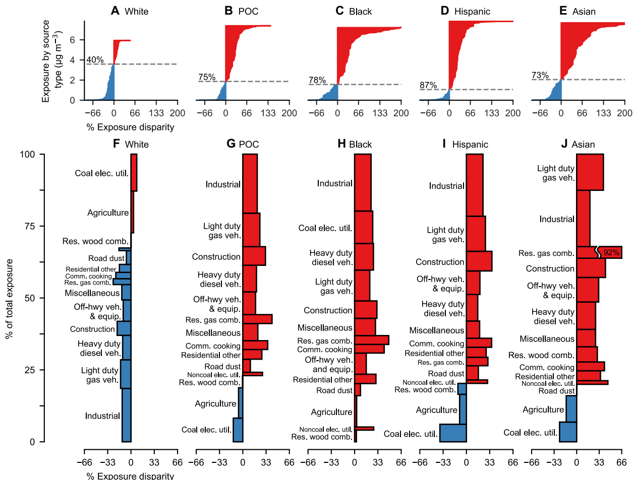
Fig. 1. Source contributions to racial-ethnic disparity in PM 2.5 exposure. (A to E) Individual source type ( n = 5434 source types) contributions to exposure (y axis) and % exposure disparity (x axis, truncated at 200%, positive values are shaded red, negative values are shaded blue), with dashed lines denoting percent exposure caused by sources with positive exposure disparity. (F to J) Sources in (A) to (E) grouped into source sectors ( n = 14 groups) and ranked vertically according to absolute exposure disparity, proportional to the area of each rectangle. As shown in (B), POC experience greater-than-average exposures from source types causing 75% of overall exposure. Source: data file S1, which also includes results for individual states and urban areas.
