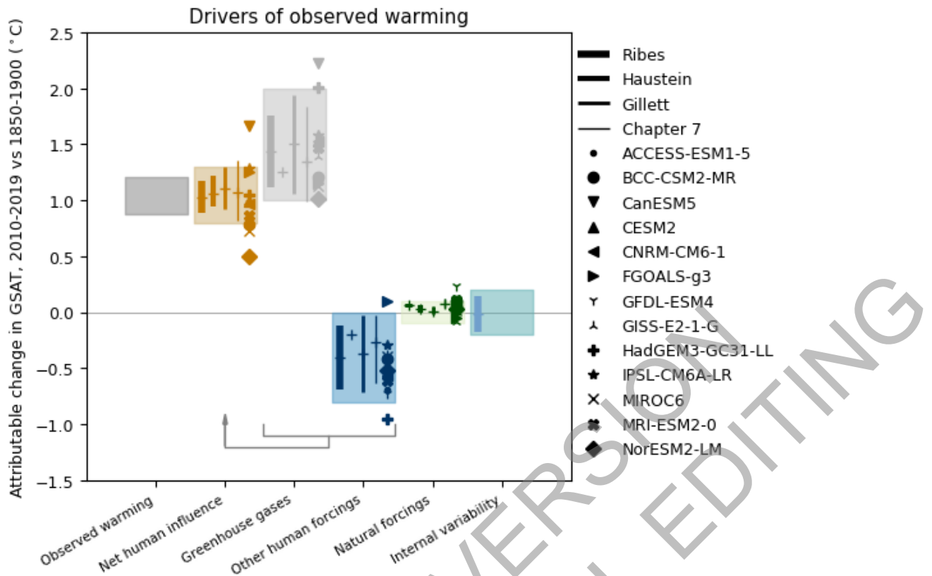
1 2 Figure 3.8: Assessed contributions to observed warming, and supporting lines of evidence. Shaded bands show 3 assessed likely ranges of temperature change in GSAT, 2010-2019 relative to 1850-1900, attributable to net 4 human influence, well-mixed greenhouse gases, other human forcings (aerosols, ozone, and land-use 5 change), natural forcings, and internal variability, and the 5-95% range of observed warming. Bars show 5- 6 95% ranges based on (left to right) Hausteine et al. (2017), Gillett et al. (2021) and Ribes et al. (2021), and 7 crosses show the associated best estimates. No 5-95% ranges were provided for the Hausteine et al. (2017) 8 greenhouse gas or other human forcings contributions. The Ribes et al. (2021) results were updated using a 9 revised natural forcing time series, and the Hausteine et al. (2017) results were updated using HadCRUT5. 10 The Chapter 7 best estimates and ranges are derived using assessed forcing time series and a two-layer 11 energy balance model as described in Section 7.3.5.3. Coloured symbols show the simulated responses to 12 the forcings concerned in each of the models indicated. Further details on data sources and processing are 13 available in the chapter data table (Table 3.SM.1). 14
