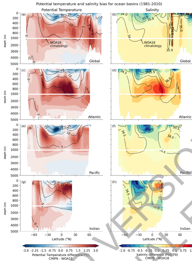
Figure 3.25: CMIP6 potential temperature and salinity biases for the global ocean, Atlantic, Pacific and Indian Oceans. Shown in colour are the time-mean differences between the CMIP6 historical multi-model climatological mean and observations, zonally averaged for each basin (excluding marginal and regional seas). The observed climatological values are obtained from the World Ocean Atlas 2018 (WOA18, 1981-2010; Prepared by the Ocean Climate Laboratory, National Oceanographic Data Center, Silver Spring, MD, USA), and are shown as labelled black contours for each of the basins. The simulated annual mean climatologies for 1981 to 2010 are calculated from available CMIP6 historical simulations, and the WOA18 climatology utilized synthesized observed data from 1981 to 2010. A total of 30 available CMIP6 models have contributed to the temperature panels (left column) and 28 models to the salinity panels (right column). Potential temperature units are °C and salinity units are the Practical Salinity Scale 1978 [PSS-78]. Further details on data sources and processing are available in the chapter data table (Table 3.SM.1).
