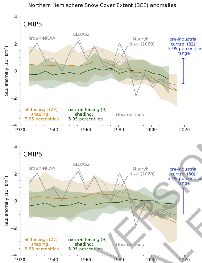
Figure 3.22: Time series of Northern Hemisphere March-April mean snow cover extent (SCE) from observations, CMIP5 and CMIP6 simulations. The observations (grey lines) are updated Brown-NOAA (Brown and Robinson, 2011), Mudryk et al. (2020), and GLDAS2. CMIP5 (upper) and CMIP6 (lower) simulations of the response to natural plus anthropogenic forcing are shown in orange, natural forcing only in green, and the pre-industrial control simulation range is presented in blue. 5-year mean anomalies are shown for the 1923-2017 period with the x-axis representing the centre years of each 5-year mean. CMIP5 all forcing simulations are extended by using RCP4.5 scenario simulations after 2005 while CMIP6 all forcing simulations are extended by using SSP2-4.5 scenario simulations after 2014. Shading indicates 5 th -95 th percentile ranges for CMIP5 and CMIP6 all and natural forcings simulations, and solid lines are ensemble means, based on all available ensemble members with equal weight given to each model (Section 3.2). The blue vertical bar indicates the mean 5 th -95 th percentile range of pre-industrial control simulation anomalies, based on non-overlapping segments. The numbers in brackets indicate the number of models used. Anomalies are relative to the average over 1971-2000. For models, SCE is restricted to grid cells with land fraction \geq 50\% . Greenland is excluded from the total area summation. Figure is modified from Paik et al. (2020), their Figure 1. Further details on data sources and processing are available in the chapter data table (Table 3.SM.1).
