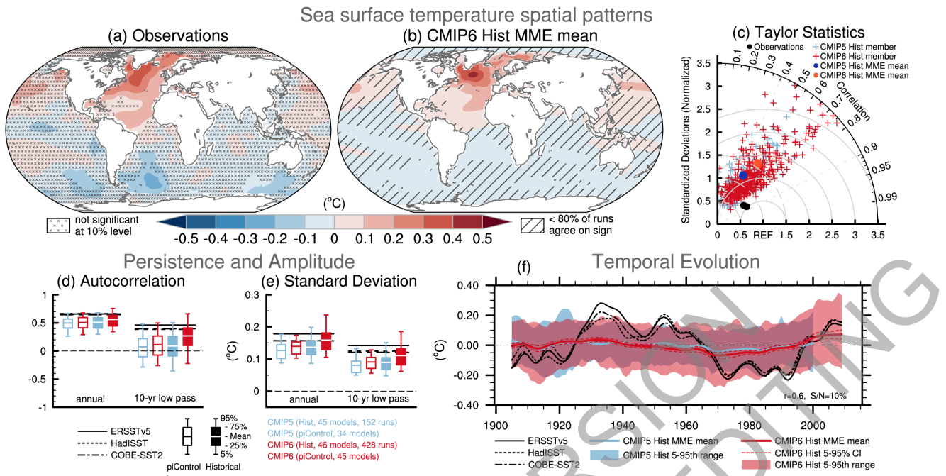
Figure 3.40: Model evaluation of Atlantic Multi-decadal Variability (AMV). (a, b) Sea surface temperature (SST) anomalies ( ^{\circ}\text{C} ) regressed onto the AMV index defined as the 10-year low-pass filtered North Atlantic ( 0^{\circ} - 60^{\circ}\text{N} , 80^{\circ}\text{W} - 0^{\circ}\text{E} ) area-weighted SST* anomalies over 1900-2014 in (a) ERSSTv5 and (b) the CMIP6 multi-model ensemble (MME) mean composite obtained by weighting ensemble members by the inverse of each model’s ensemble size. The asterisk denotes that the global mean SST anomaly has been removed at each time step of the computation. Cross marks in (a) represent regions where the anomalies are not significant at the 10% level based on a t-test. Diagonal lines in (b) show regions where less than 80% of the runs agree in sign. (c) A Taylor diagram summarizing the representation of the AMV pattern in CMIP5 (each member is shown as a cross in light blue, and the weighted multi-model mean is shown as a dot in dark blue), CMIP6 (each member is shown as a cross in red, and the weighted multi-model mean is shown as a dot in orange) and observations over [ 0^{\circ} - 60^{\circ}\text{N} , 80^{\circ}\text{W} - 0^{\circ}\text{E} ]. The reference pattern is taken from ERSSTv5 and black dots indicate other observational products (HadISSTv1 and COBE-SST2). (d) Autocorrelation of unfiltered annual AMV index at lag 1 year and 10-year low-pass filtered AMV index at lag 10 years for observations over 1900-2014 (horizontal lines) and 115-year chunks of pre-industrial control simulations (open boxes) and individual historical simulations over 1900-2014 (filled boxes) from CMIP5 (blue) and CMIP6 (red). (e) As in (d), but showing standard deviation of the unfiltered and filtered AMV indices ( ^{\circ}\text{C} ). Boxes and whiskers show the weighted multi-model mean, interquartile ranges and 5 th and 95 th percentiles. (f) Time series of the AMV index ( ^{\circ}\text{C} ) in ERSSTv5, HadISSTv1 and COBE-SST2 observational estimates (black) and CMIP5 and CMIP6 historical simulations. The thick red and light blue lines are the weighted multi-model mean for the historical simulations in CMIP5 and CMIP6, respectively, and the envelopes represent the 5 th -95 th percentile range obtained from all ensemble members. The 5-95% confidence interval for the CMIP6 multi-model mean is shown by the thin dashed line. Further details on data sources and processing are available in the chapter data table (Table 3.SM.1).
