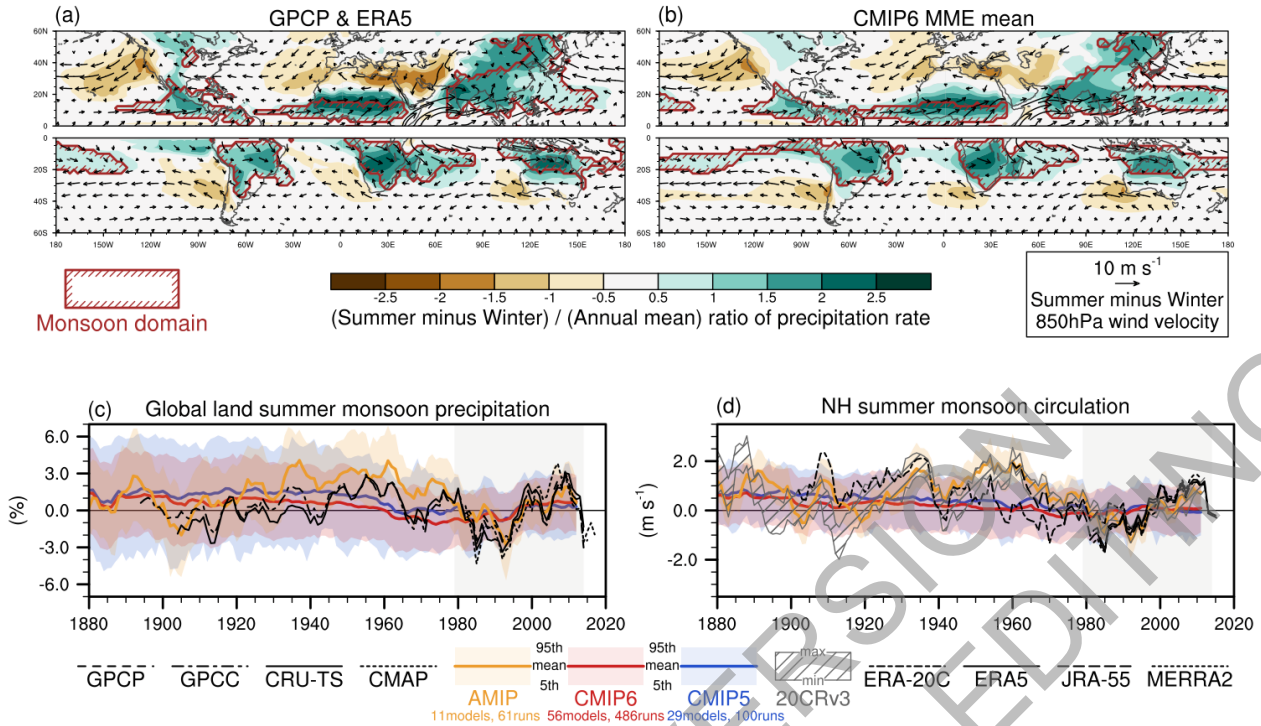
Figure 3.17: Model evaluation of global monsoon domain, intensity, and circulation. (a-b) Climatological summer-winter range of precipitation rate, scaled by annual mean precipitation rate (shading) and 850 hPa wind velocity (arrows) based on (a) GPCP and ERA5 and (b) a multi-model ensemble mean of CMIP6 historical simulations for 1979-2014. Enclosed by red lines is the monsoon domain based on the definition by Wang and Ding (2008). (c-d) 5-year running mean anomalies of (c) global land monsoon precipitation index defined as the percentage anomaly of the summertime precipitation rate averaged over the monsoon regions over land, relative to its average for 1979-2014 (the period indicated by light grey shading) and (d) the tropical monsoon circulation index defined as the vertical shear of zonal winds between 850 and 200 hPa levels averaged over 0°-20°N, from 120°W eastward to 120°E in NH summer (Wang et al., 2013; m s -1 ) in CMIP5 historical and RCP4.5 simulations, CMIP6 historical and AMIP simulations. Summer and winter are defined for individual hemispheres: May through September for NH summer and SH winter, and November through March for NH winter and SH summer. The number of models and ensembles are given in the legend. The multi-model ensemble mean and percentiles are calculated after weighting individual members with the inverse of the ensemble size of the same model, so that individual models are equally weighted irrespective of ensemble size. Further details on data sources and processing are available in the chapter data table (Table 3.SM.1).
