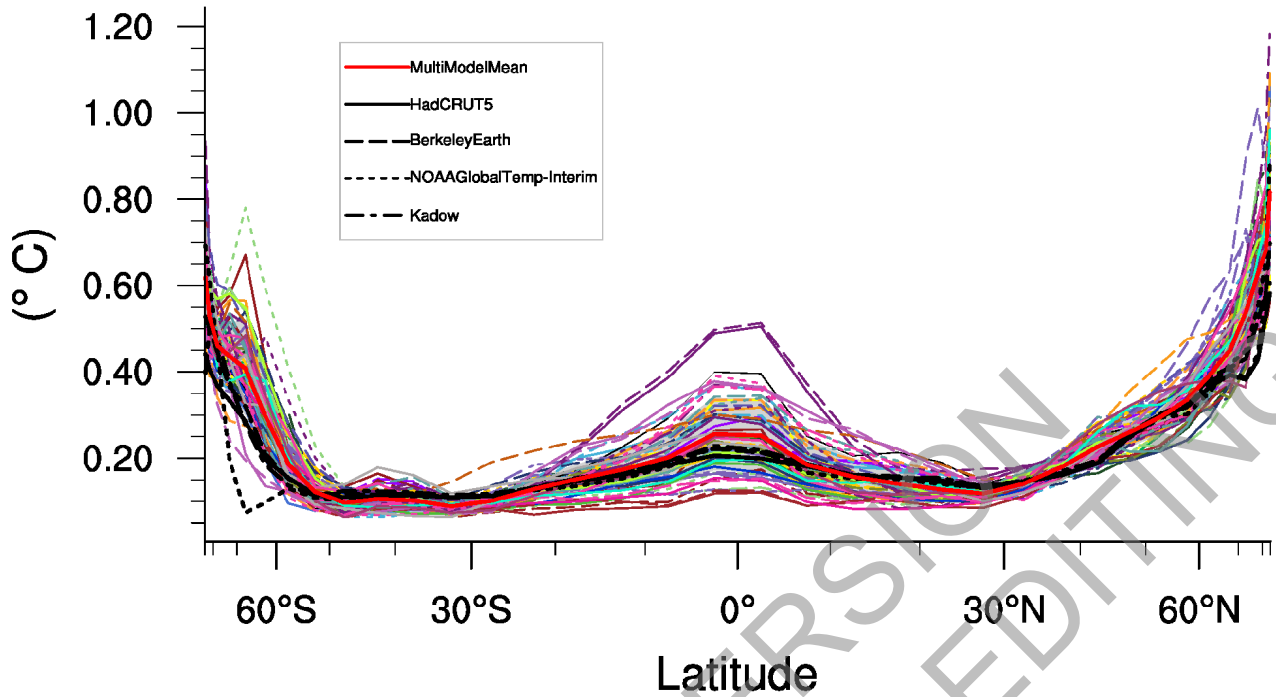
Figure 3.5: The standard deviation of annually averaged zonal-mean near-surface air temperature. This is shown for four detrended observed temperature datasets (HadCRUT5, Berkeley Earth, NOAAGlobalTemp-Interim and Kadow et al. (2020), for the years 1995-2014) and 59 CMIP6 pre-industrial control simulations (one ensemble member per model, 65 years) (after Jones et al., 2013). For line colours see the legend of Figure 3.4. Additionally, the multi-model mean (red) and standard deviation (grey shading) are shown. Observational and model datasets were detrended by removing the least-squares quadratic trend. Further details on data sources and processing are available in the chapter data table (Table 3.SM.1).
