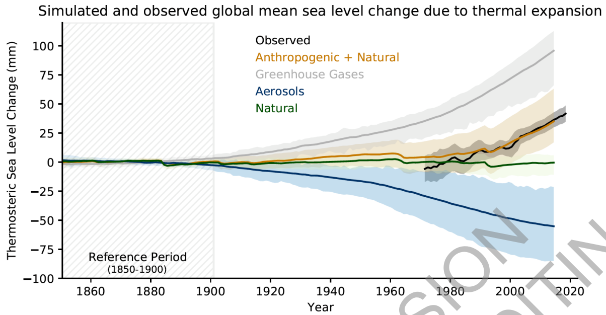
Figure 3.29: Simulated and observed global mean sea level change due to thermal expansion for CMIP6 models and observations relative to the baseline period 1850-1900. Historical simulations are shown in brown, natural only in green, greenhouse gas only in grey, and aerosol only in blue (multi-model means shown as thick lines, and shaded ranges between the 5 th and 95 th percentile). The best estimate observations (black solid line) for the period of 1971-2018, along with very likely ranges (black shading) are from Section 2.3.3.1 and are shifted to match the multi-model mean of the historical simulations for the 1995-2014 period. Further details on data sources and processing are available in the chapter data table (Table 3.SM.1).
