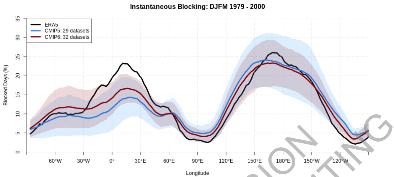
1 2 Figure 3.18: Instantaneous Northern-Hemisphere blocking frequency (% of days) in the extended northern 3 winter season (DJFM) for the years 1979-2000. Results are shown for ERA5 reanalysis (black), CMIP5 4 (blue) and CMIP6 (red) models. Coloured lines show multi-model means and shaded ranges show 5 corresponding 5-95% ranges constructed with one realization from each model. Figure is adapted from 6 Davini and D'Andrea (2020), their Figure 12 and following the D'Andrea et al. (1998) definition of 7 blocking. Further details on data sources and processing are available in the chapter data table (Table 8 3.SM.1). 9
