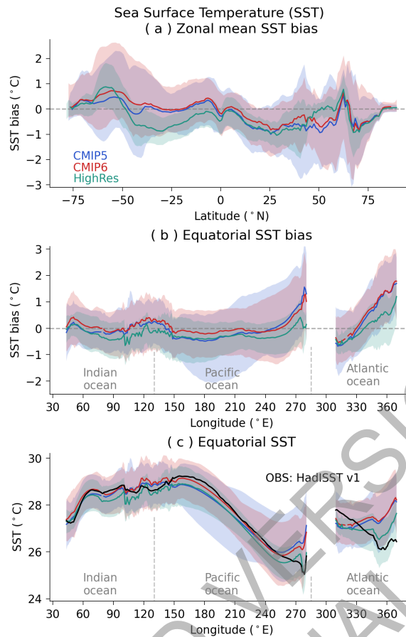
Figure 3.24: Biases in zonal mean and equatorial sea surface temperature (SST) in CMIP5 and CMIP6 models. CMIP6 (red), CMIP5 (blue) and HighResMIP (green) multi-model mean (a) zonally-averaged SST bias; (b) equatorial SST bias; and (c) equatorial SST compared to observed mean SST (black line) for 1979-1999. The inter-model 5th and 95th percentiles are depicted by the respective shaded range. Model climatologies are derived from the 1979-1999 mean of the historical simulations, using one simulation per model. The Hadley Centre Sea Ice and Sea Surface Temperature version 1 (HadISST) (Rayner et al., 2003) observational climatology for 1979-1999 is used as the reference for the error calculation in (a) and (b); and for observations in (c). Further details on data sources and processing are available in the chapter data table (Table 3.SM.1).
