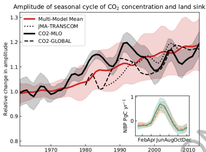
1 2 Figure 3.32: Relative change in the amplitude of the seasonal cycle of global land carbon uptake in the historical 3 CMIP6 simulations from 1961-2014. Net biosphere production estimates from 19 CMIP6 models (red), 4 the data-led reconstruction JMA-TRANSCOM (Maki et al., 2010; dotted) and atmospheric CO 2 seasonal 5 cycle amplitude changes from observations (global as dashed line, Mauna Loa Observatory (MLO) 6 (Dlugokencky et al., 2020) in bold black). Seasonal cycle amplitude is calculated using the curve fit 7 algorithm package from the National Oceanic and Atmospheric Administration Earth System Research 8 Laboratory (NOAA ESRL). Relative changes are referenced to the 1961-1970 mean and for short time 9 series adjusted to have the same mean as the model ensemble in the last 10 years. Interannual variation 10 was removed with a 9-year Gaussian smoothing. Shaded areas show the one sigma model spread (grey) 11 for the CMIP6 ensemble and the one sigma standard deviation of the smoothing (red) for the CO 2 MLO 12 observations. Inset: average seasonal cycle of ensemble mean net biosphere production and its one sigma 13 model spread for 1961-1970 (orange dashed line, light orange shading) and 2005-2014 (solid green line, 14 green shading). Further details on data sources and processing are available in the chapter data table 15 (Table 3.SM.1). 16
