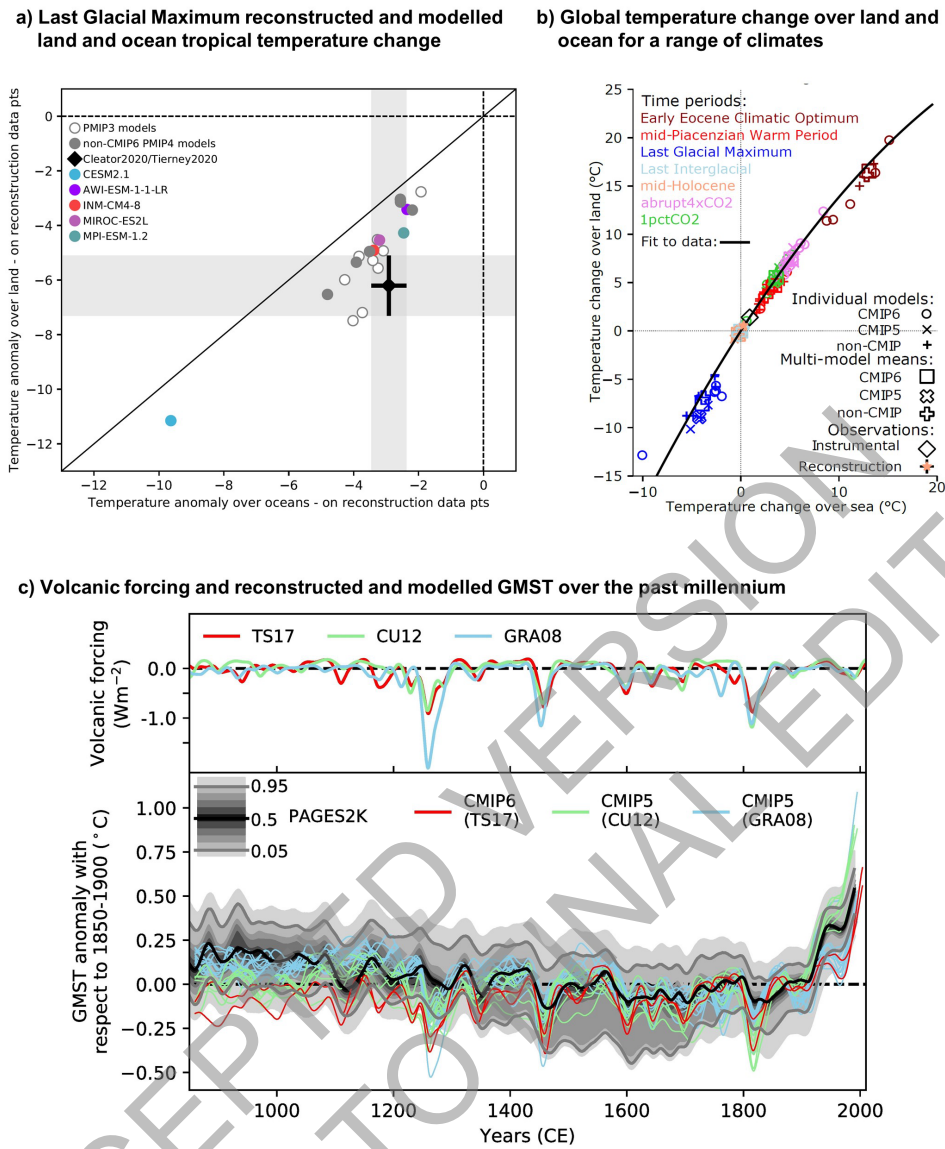
1 2 Figure 3.2: Changes in surface temperature for different paleoclimates. (a) Comparison of reconstructed and 3 modelled surface temperature anomalies for the Last Glacial Maximum over land and ocean in the Tropics 4 (30°N to 30°S). Land-based reconstructions are from Cleator et al., (2020). Ocean-based reconstructions 5 are from Tierney et al. (2020). Model points are calculated as the difference between Last Glacial 6 Maximum and pre-industrial control simulations of the PMIP3 and PMIP4 ensembles, sampled at the 7 reconstruction data points. (b) Land-sea contrast in global mean surface temperature change for different 8 paleoclimates. Crosses show individual model simulations from the CMIP5 and CMIP6 ensembles. Filled 9 symbols show ensemble means and assessed values. Acronyms are LGM Last Glacial Maximum, LIG Last 10 Inter Glacial, MPWP mid-Pliocene Warm Period, EECO Early Eocene Climatic Optimum. (c) Upper panel 11 shows time series of volcanic radiative forcing, in W m^{-2} , as used in the CMIP5 (Gao et al., 2008; Crowley 12 and Unterman, 2013; see also Schmidt et al., 2011) and CMIP6 (850 BCE to 1900 CE from Toohey and 13 Sigl (2017), 1850-2015 from Luo (2018)). The forcing has been calculated from the stratospheric aerosol 14 optical depth at 550 nm shown in Figure 2.2. Lower panel shows time series of global mean surface 15 temperature anomalies, in K, with respect to 1850-1900 for the CMIP5 and CMIP6 past1000 simulations 16 and their historical continuation simulations. Simulations are coloured according to the volcanic radiative 17 forcing dataset they used. The temperature median reconstruction by PAGES 2k Consortium (2019) is 18 shown in black, the 5-95% confidence interval by grey lines and the grey envelopes show the 1, 5, 15, 25, 19 35, 45, 55, 65, 75, 85, 95, and 99 percentiles. All data in both panels are band-passed, where frequencies 20 longer than 20 years have been retained. Further details on data sources and processing are available in the 21 chapter data table (Table 3.SM.1).
