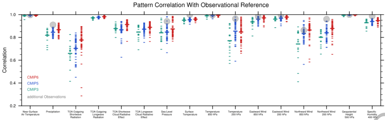
Figure 3.43: Centred pattern correlations between models and observations for the annual mean climatology over the period 1980–1999. Results are shown for individual CMIP3 (cyan), CMIP5 (blue) and CMIP6 (red) models (one ensemble member from each model is used) as short lines, along with the corresponding ensemble averages (long lines). Correlations are shown between the models and the primary reference observational data set (from left to right: ERA5, GPCP-SG, CERES-EBAF, CERES-EBAF, CERES-EBAF, CERES-EBAF, JRA-55, ESACCI-SST, ERA5, ERA5, ERA5, ERA5, ERA5, ERA5, AIRS, ERA5). In addition, the correlation between the primary reference and additional observational data sets (from left to right: NCEP, GHCN, -, -, -, ERA5, HadISST, NCEP, NCEP, NCEP, NCEP, NCEP, NCEP, ERA5, NCEP) are shown (solid grey circles) if available. To ensure a fair comparison across a range of model resolutions, the pattern correlations are computed after regridding all datasets to a resolution of 4° in longitude and 5° in latitude. Figure is updated and expanded from Bock et al. (2020), their Figure 7 CC BY4.0 https://creativecommons.org/licenses/by/4.0/ . Further details on data sources and processing are available in the chapter data table (Table 3.SM.1
