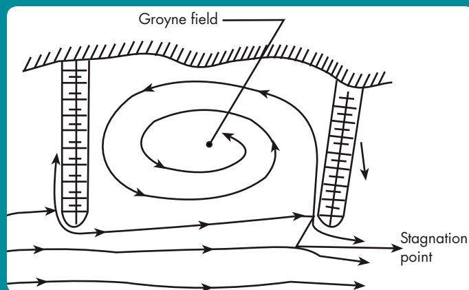
Figure 49: Formation of eddy between two spurs
