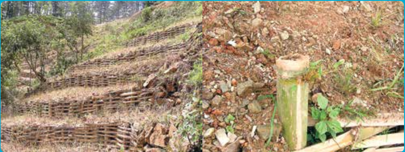
Figure 8: Bamboo fencing on a slope – the posts (pegs) are live bamboo that will sprout to provide foliage (left); detail showing live bamboo peg with sprouting leaves (right)
