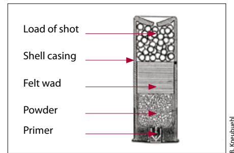
Figure 3.8 Shotgun shell and load of shot.
