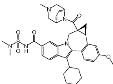
Beclabuvir
